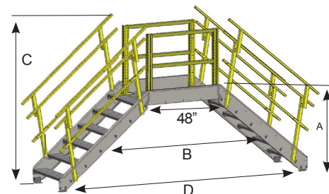
Stair Crossover Bridge
