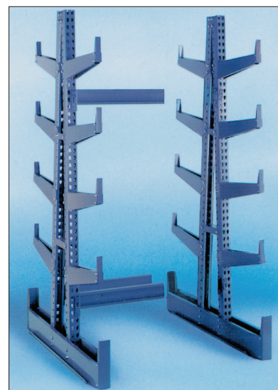
Double-faced Rack Add-on
