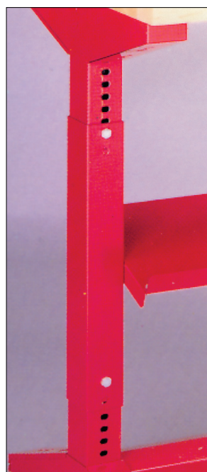
Fully Adjustable Leg heights from 26" to 44" in 1/2" increments.
