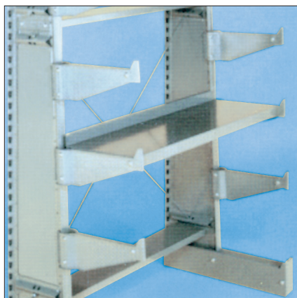
Shelves (12" x 36") fit between rack arms to hold long and short products in same unit.
